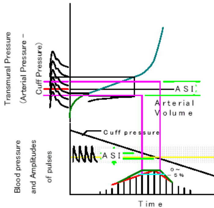
Fig. 1 Schematic diagram illustrating the principle for the determination of arterial stiffness index.
